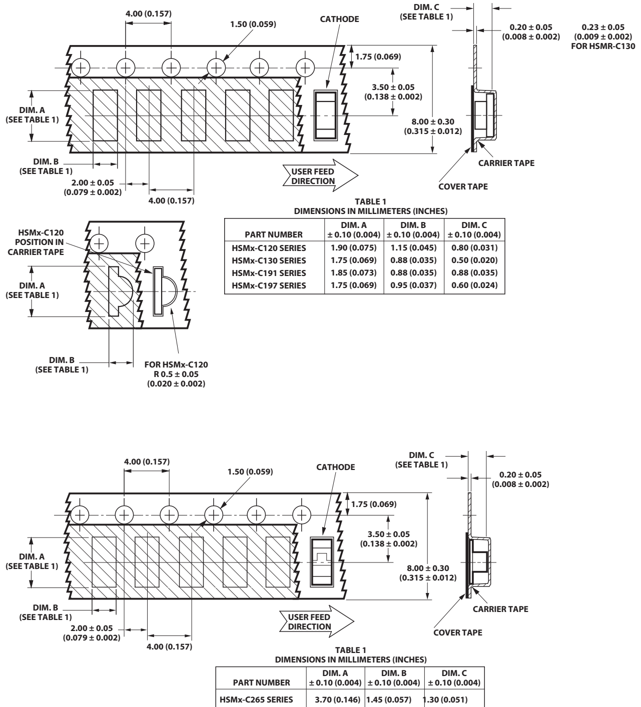
Figure 17. Tape dimensions.
